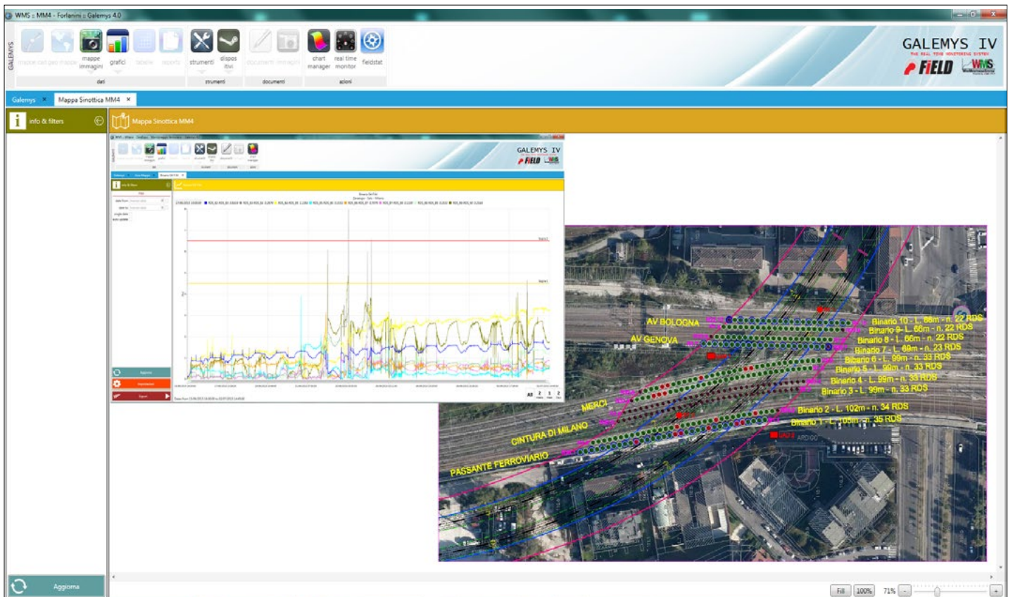
This WMS screen shot shows the position of the RDS gauges on job site with nine tracks where an underpass is being constructed. The plot represents the railway twisting. Alert and alarm thresholds are represented by straight yellow and red lines.
