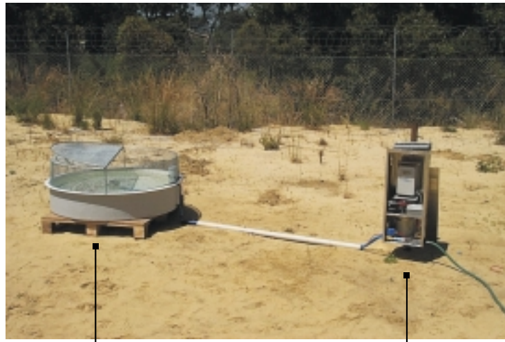
Evaporation pan with bird guard
